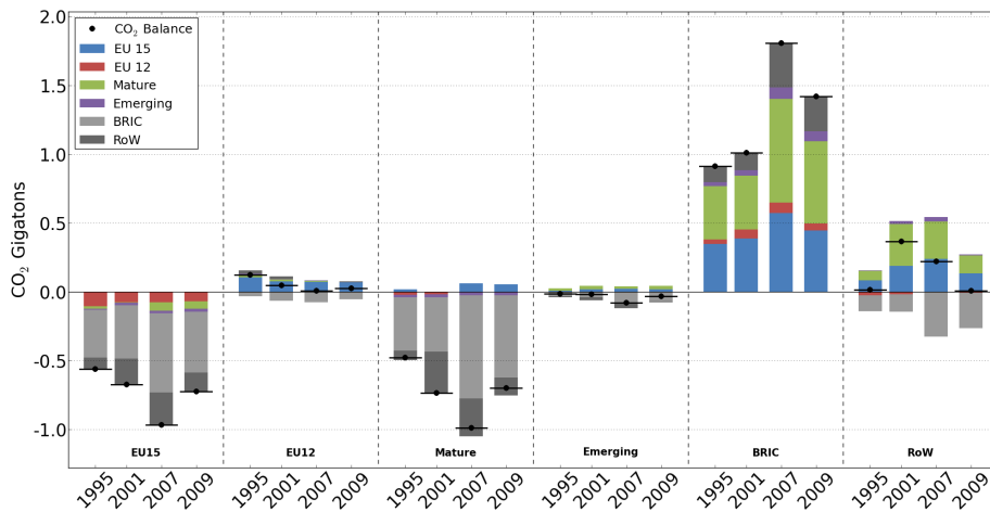
Figure 4: Carbon balances in CO 2 Gigatons
