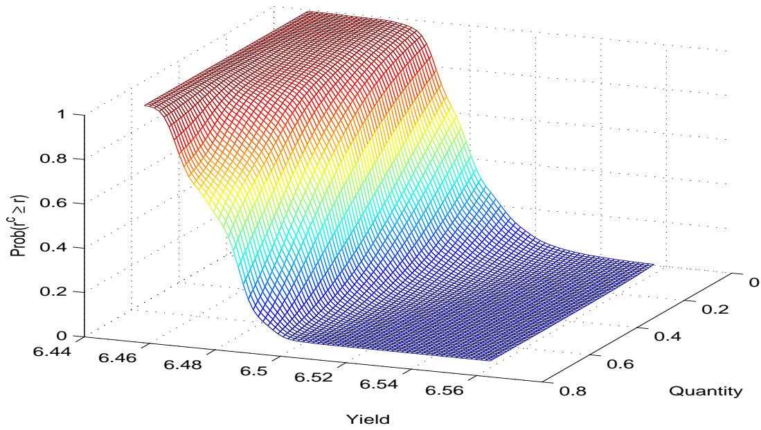
Figure 6: Bidder valuations: Auction 21, Bidder 35
