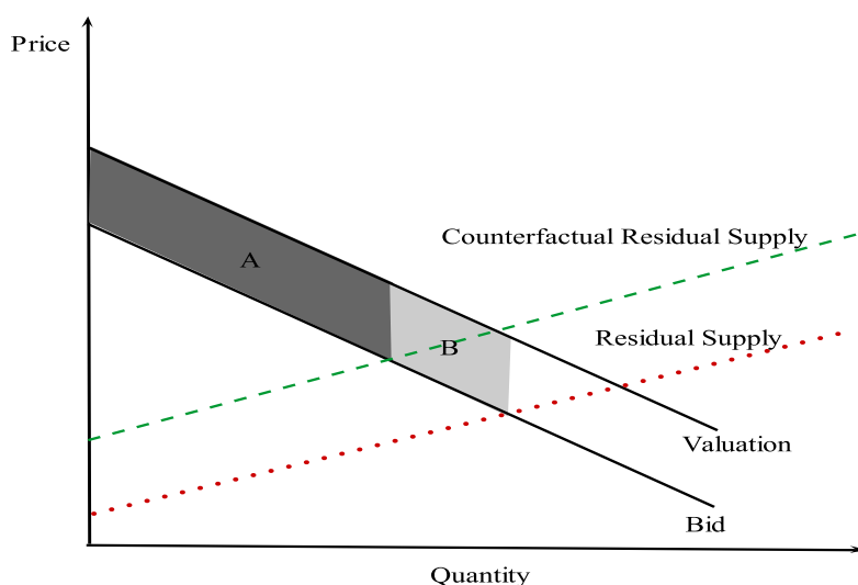
Figure 9: Statistical effect
