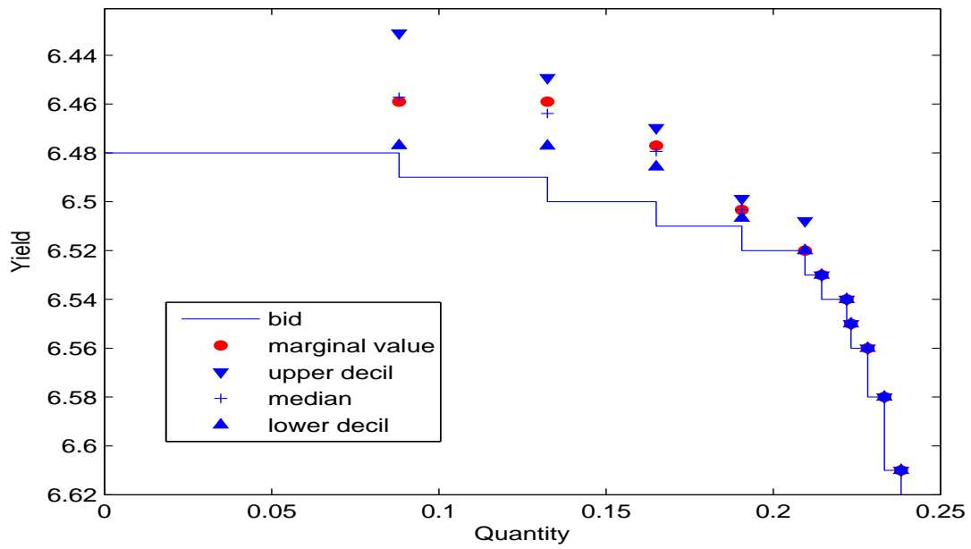
Figure 6: Bidder valuations: Auction 21, Bidder 35
